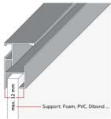
Mounting example of conventional assembly
